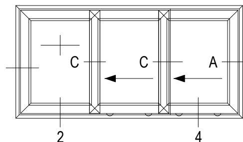
ELEVATION VIEW EXTERIOR SIDE
