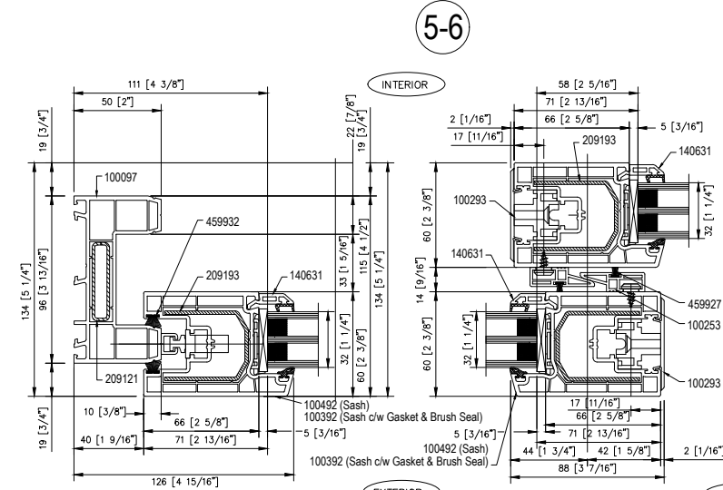
D Right cross section: Sliding door sash - outside
