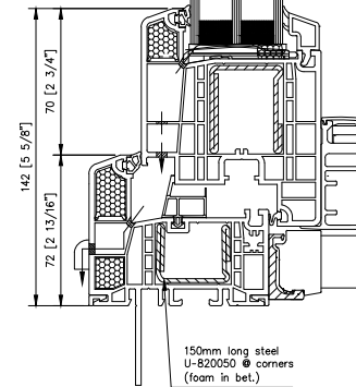
4 4700 TILT & GLIDE - SILL
