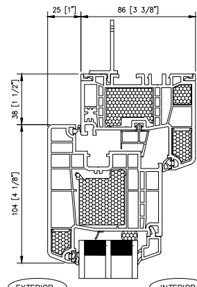
1 4700 OUTSWING - HEAD
