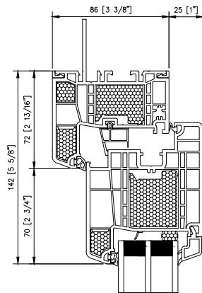
1 4700 INSWING - HEAD
