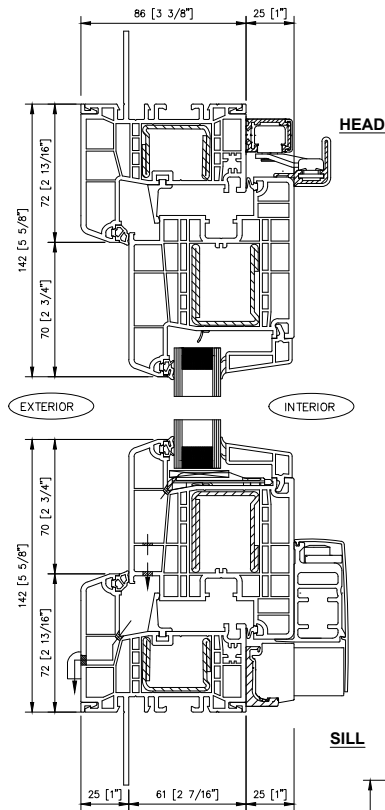
4 4700 TILT & GLIDE - SILL
