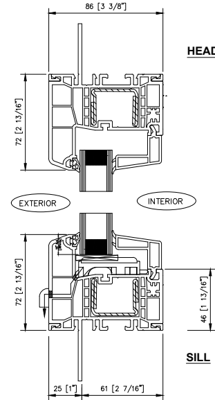
3 4700 SIDELITE - HEAD
