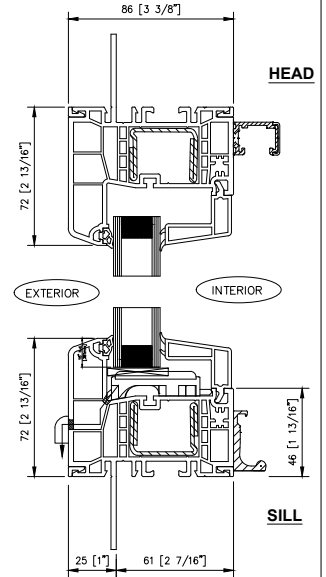
7 4700 SIDELITE - HEAD
