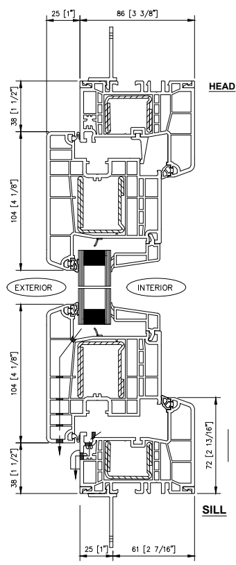
2 4700 OUTSWING - SILL
