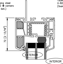
3 4700 SIDELITE - HEAD
