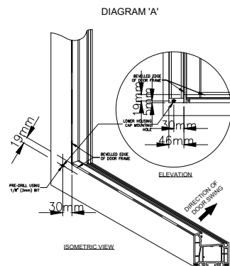
INSWING & OUTSWING FRENCH DOOR
