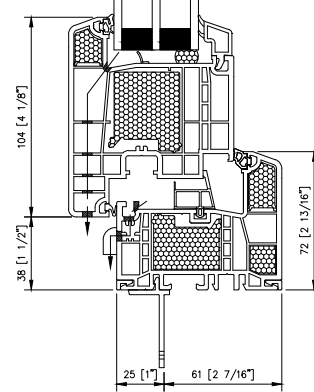
2 4700 OUTSWING - SILL
