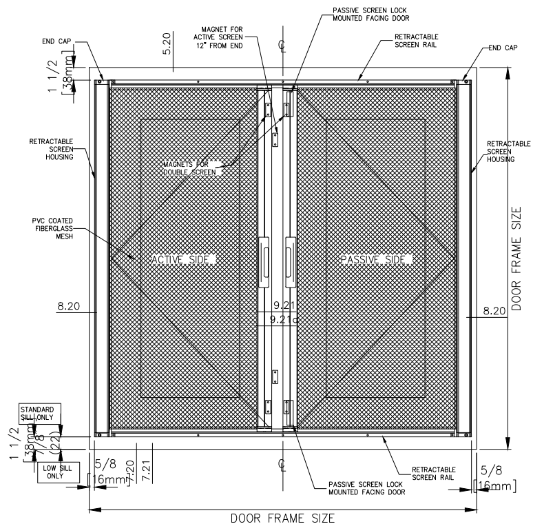
INSWING & OUTSWING FRENCH DOOR
