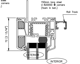
7 4700 SIDELITE - HEAD
