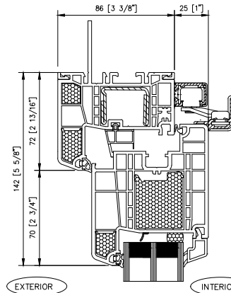
3 4700 TILT & GLIDE - HEAD
