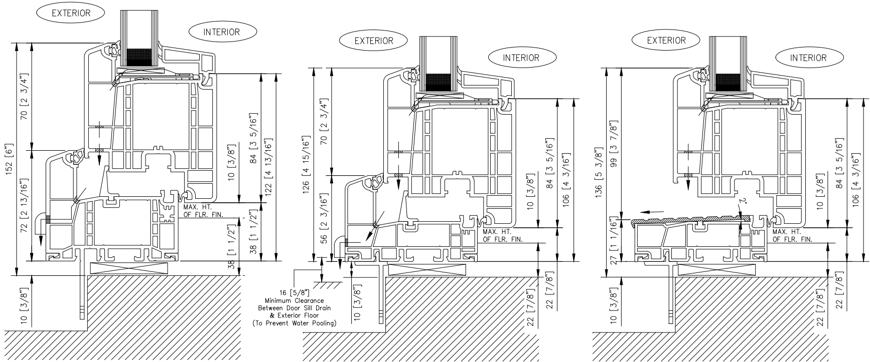
STANDARD SILL
